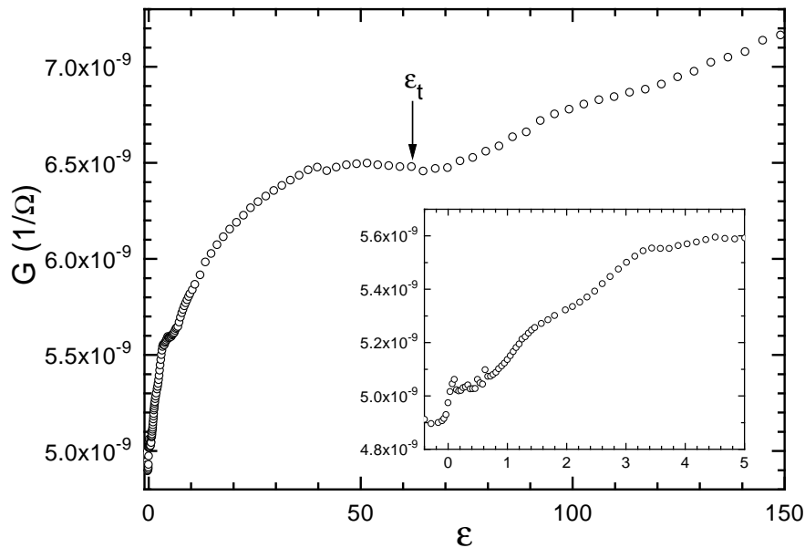
FIG. 11. Voltage dependence of the conductivity G in conductive EHC ( T = 50^\circ\text{C} , f = 100\text{Hz} ) obtained from long-time fluctuation measurements. Inset: blowup of the low voltage region.
