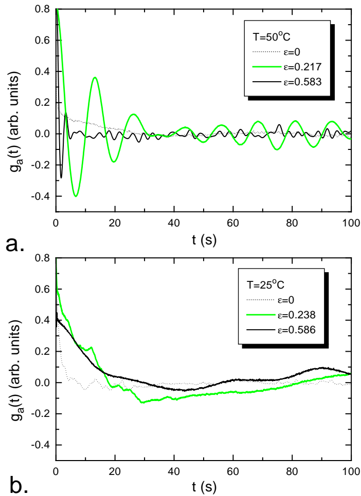
FIG. 6. Autocorrelation functions g_a(t) at similar values of \epsilon in the conductive- (a) and in the dielectric regime (b) of EHC.
