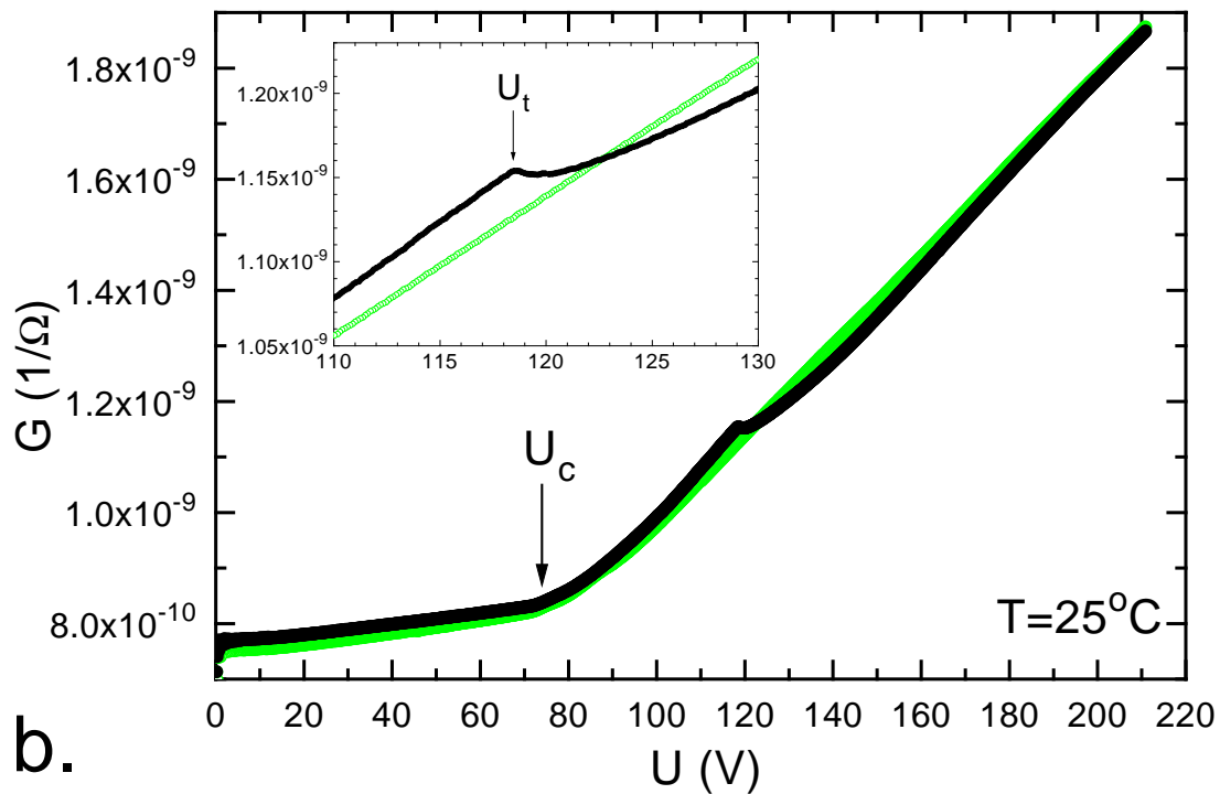
FIG. 2. Conductivity G vs. the applied voltage U in a cycle with increased voltage steps (black, closed symbols) followed by decreased voltage steps (gray, open symbols) at: (a) T = 50^\circ\text{C} (conductive regime of EHC) and at (b) T = 25^\circ\text{C} (dielectric regime). The inset shows blow-up of the voltage range where the anisotropic – isotropic turbulence transition takes place.
