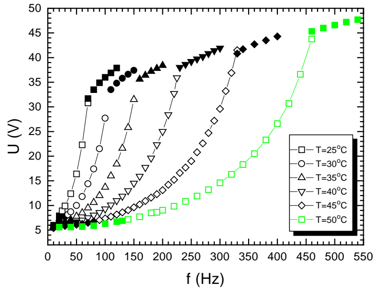
FIG. 1. Phase diagram of EHC at different temperatures T . The closed symbols in the low frequency range denote stationary (normal or oblique) rolls. Open symbols stand for the non-stationary, travelling rolls and in the high frequency range the closed symbols are for dielectric normal rolls.
