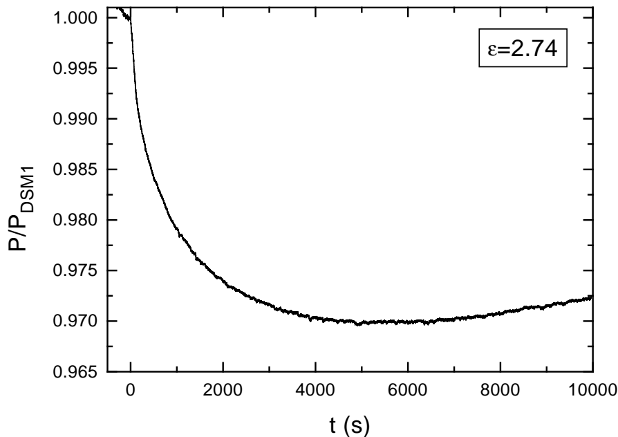
FIG. 9. Temporal dependence of the injected power P in DSM2 (dielectric EHC) turbulence normalized with P_{\text{DSM1}} measured in DSM1. The DSM1 – DSM2 transition takes place at t = 0 ; T = 25^\circ\text{C} ; \varepsilon = 2.74 (> \varepsilon_t) .
