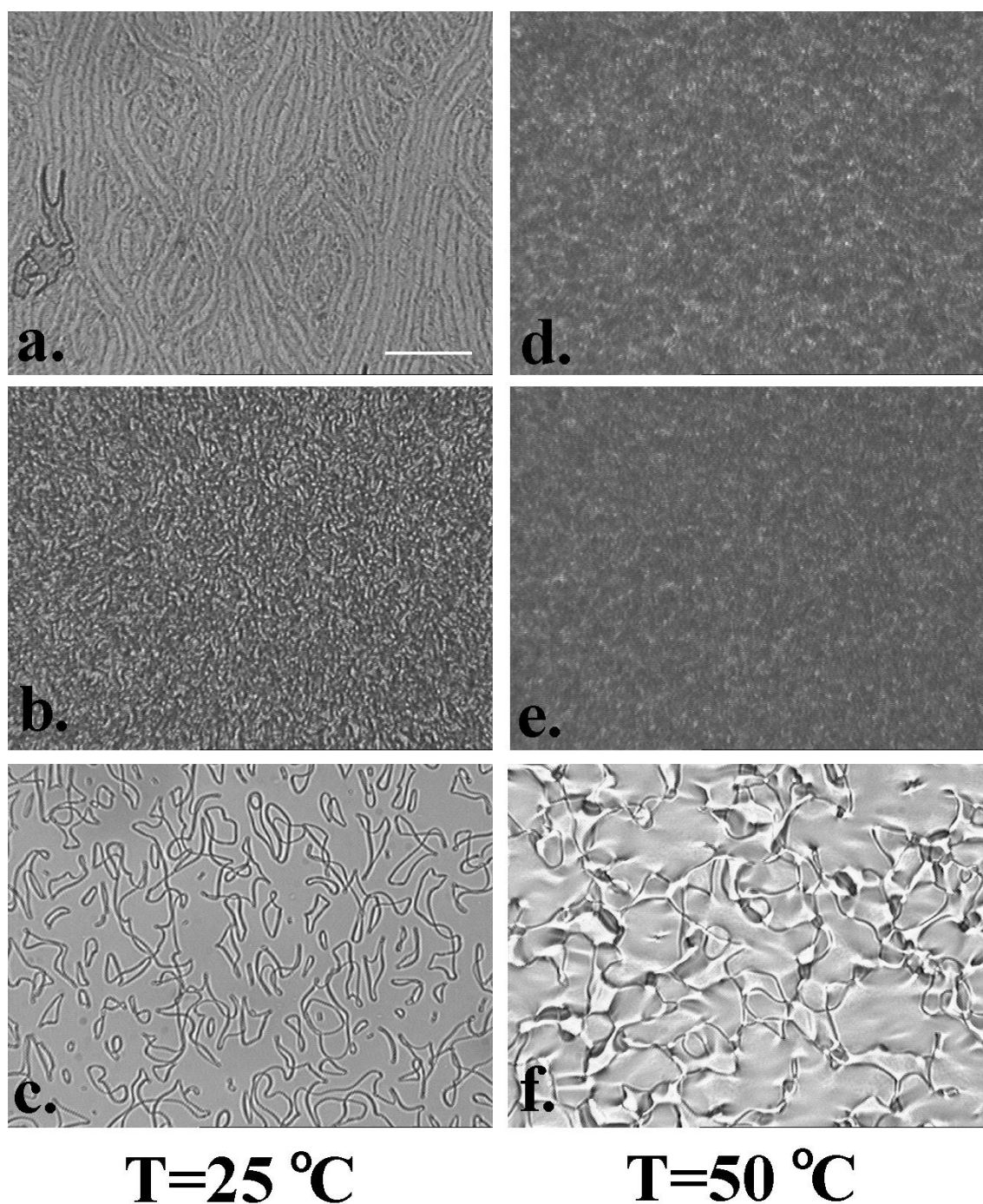
FIG. 12. Snapshots of DSM1 [(a) and (d)], DSM2 [(b) and (e)] patterns as well as the images of the disclination loops taken immediately after switching off the driving voltage. (a)–(c) dielectric EHC ( T = 25^\circ\text{C} , \varepsilon = 2.7 ); (d)–(f) conductive EHC ( T = 50^\circ\text{C} , \varepsilon = 62.1 ). The scale bar in subfigure (a) shows 100\mu\text{m} .
