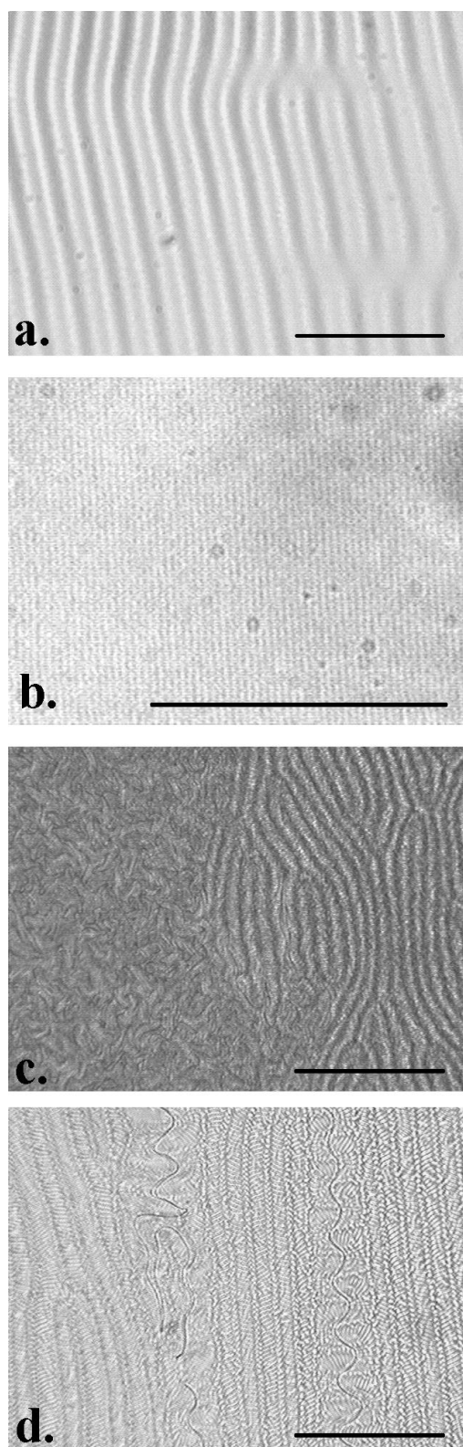
FIG. 3. Snapshots of the EHC patterns at characteristic points shown in Fig. 2. (a) at T = 50^{\circ}\text{C} and at the threshold U_c = 6.97\text{V} of the oblique rolls; (b) at T = 25^{\circ}\text{C} and at the threshold U_c = 73.2\text{V} of the dielectric normal rolls; (c) at T = 25^{\circ}\text{C} and at the anisotropic – isotropic turbulence transition voltage U_t = 118.5\text{V} showing the transition front passing through the sample; (d) a demonstration of persistence of the disclination loops in the case of decreased voltage steps at T = 25^{\circ}\text{C} and U = 88.2\text{V} . The scale bars show 100\mu\text{m} .
