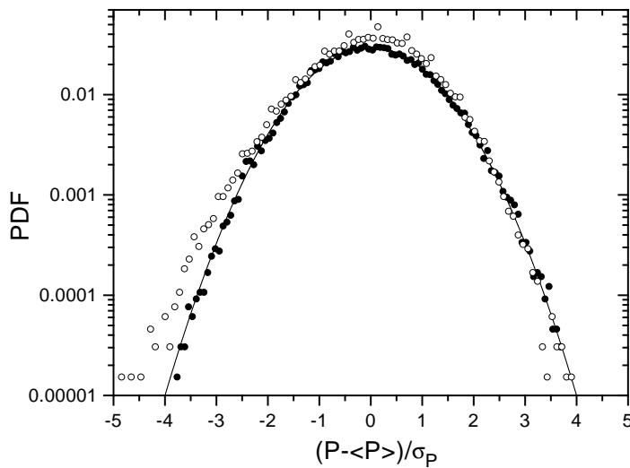
FIG. 7. Probability density function (PDF) of the power fluctuations above the onset of EHC, at \epsilon \approx 0.6 for T = 50^\circ\text{C} (conductive EHC, filled symbols) and for T = 25^\circ\text{C} (dielectric EHC, open symbols). The line shows the Gaussian distribution with no fitting parameters.
