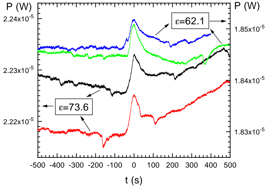
FIG. 10. Electric power vs. time near the DSM1 \rightarrow DSM2 turbulence transition (taking place around t = 0 ) in conductive EHC ( T = 50^\circ\text{C} ) for two different \varepsilon as indicated in the figure.
