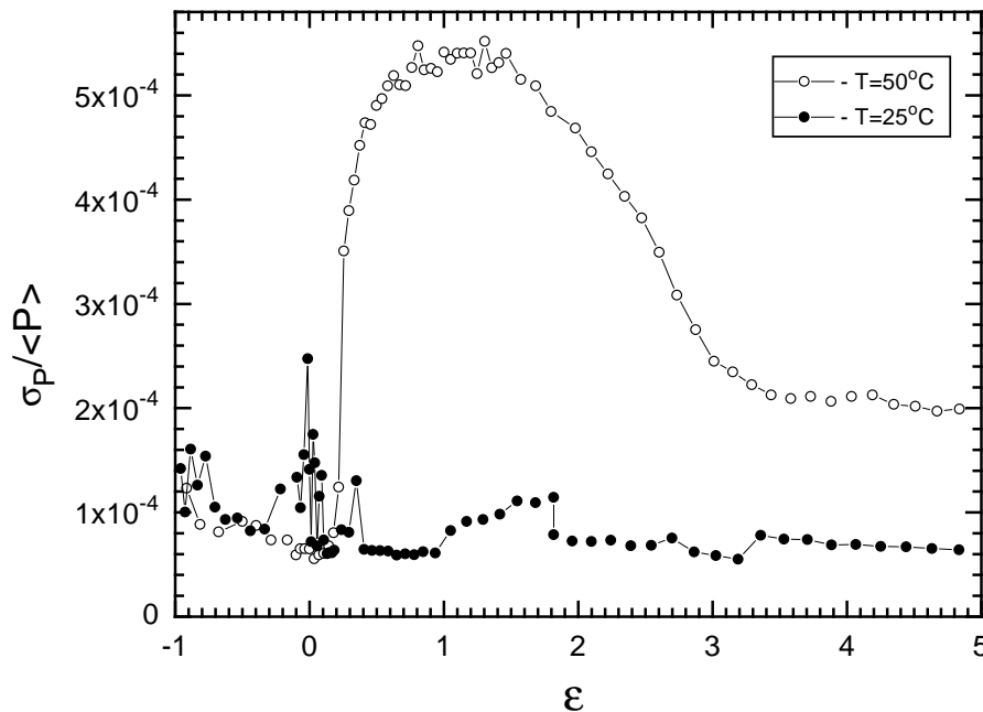
FIG. 4. The standard deviation of the power fluctuations normalised with the mean value of electric power \langle P \rangle as a function of the dimensionless driving voltage \varepsilon in the conductive regime of EHC (empty symbols) and in the dielectric regime of EHC (filled symbols).
