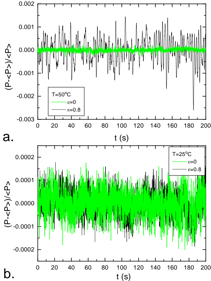
FIG. 5. Electric power fluctuations at same values of voltage \varepsilon in the conductive (a) and dielectric regime of EHC (b).
